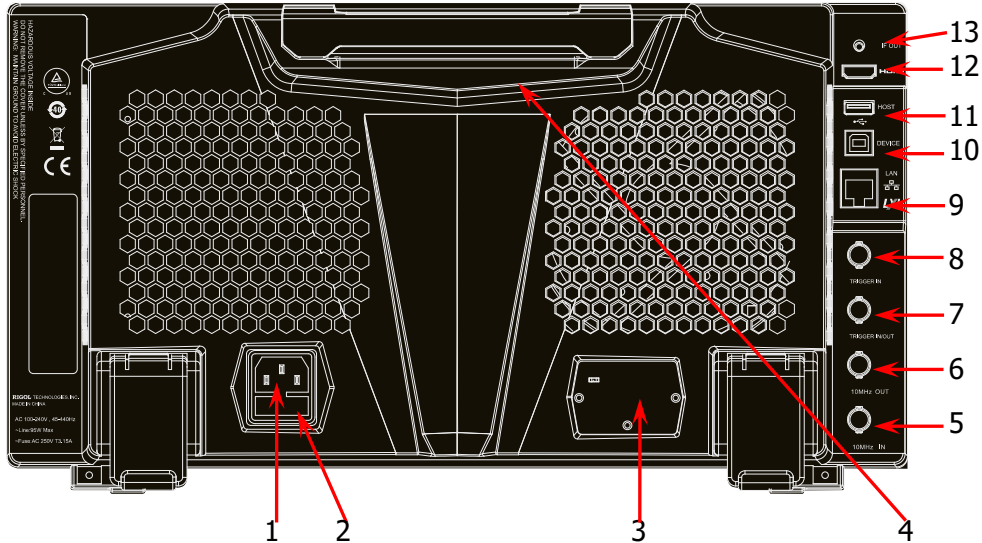
Figure 1-8 Rear Panel
