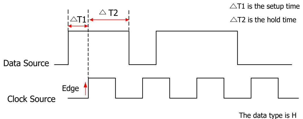
Figure 8.11 Setup/Hold Trigger
