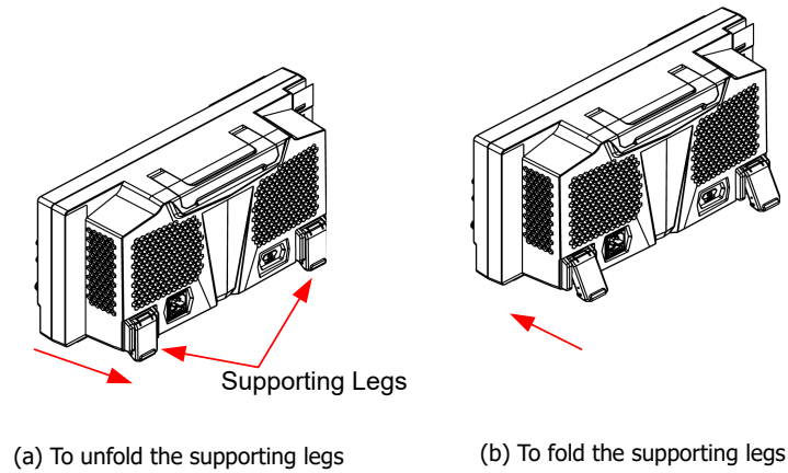
Figure 4.3 To Adjust the Supporting Legs
