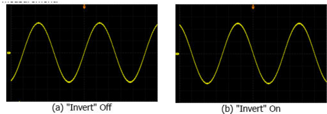
Figure 5.1 Waveform Invert
