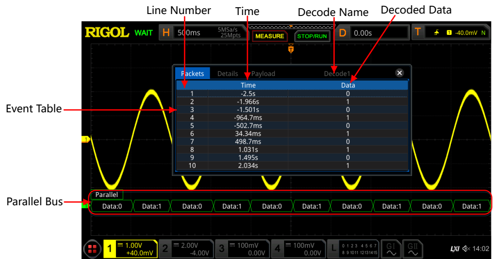
Figure 15.2 Parallel Decoding Event Table
