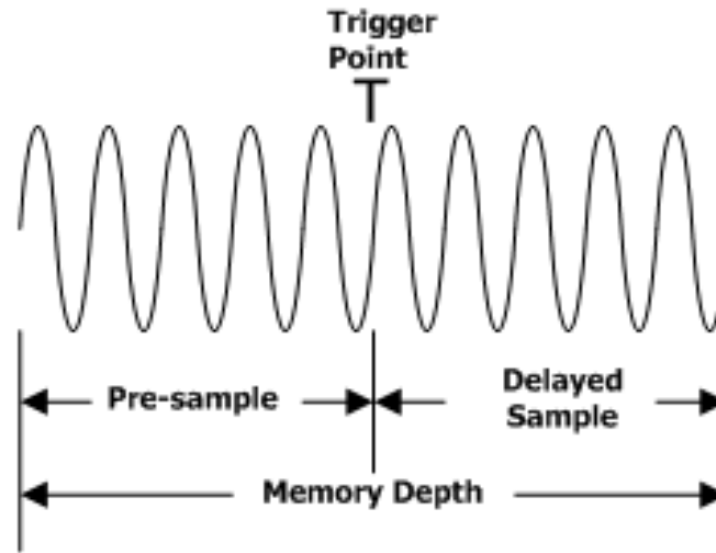
Figure 7.4 Memory Depth
