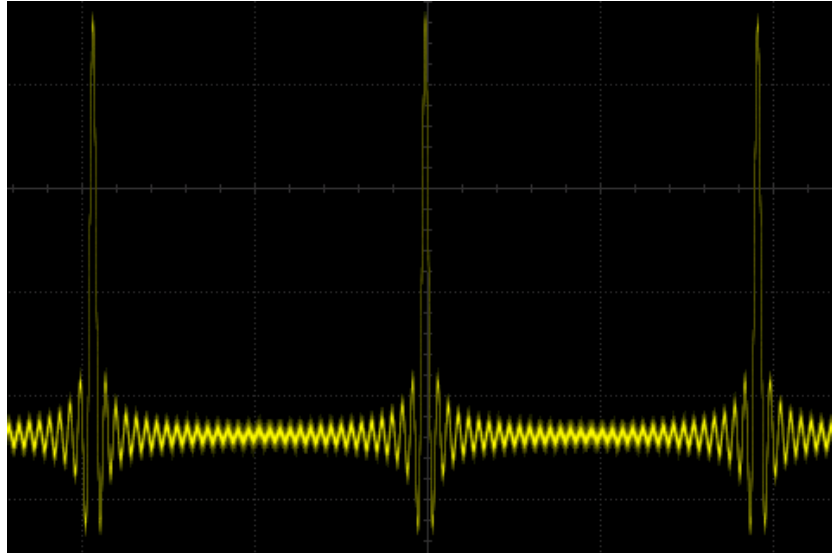
Figure 21.3 Sinc
