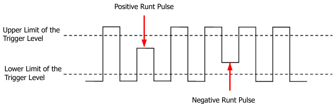
Figure 8.9 Runt Trigger
