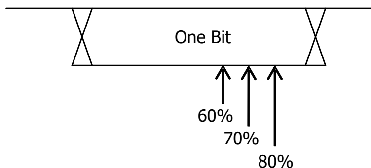
Figure 15.10 Sample Position
