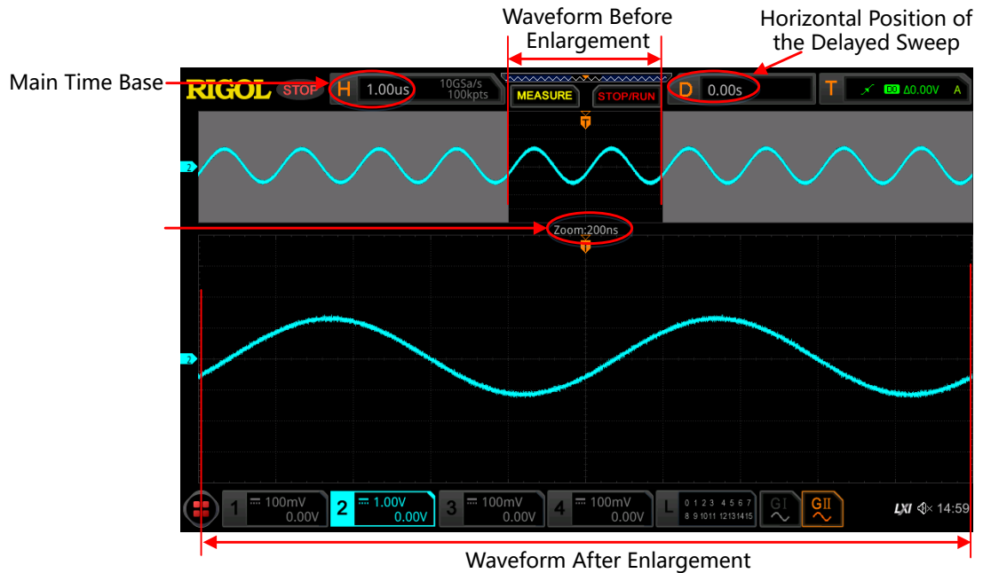
Figure 6.1 Delayed Sweep Mode
