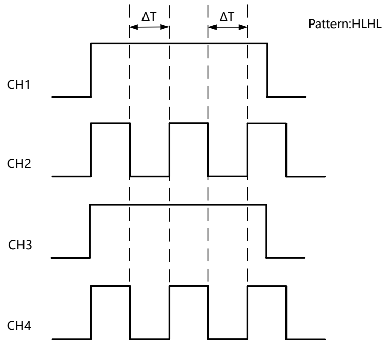
Figure 8.7 Duration Trigger
