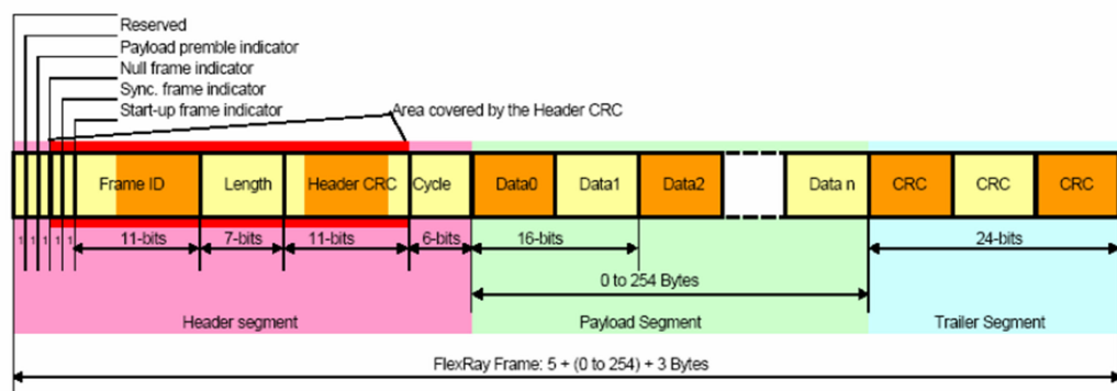
Figure 8.20 Frame Format of FlexRay Bus
