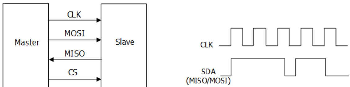
Figure 15.7 SPI Serial Bus
