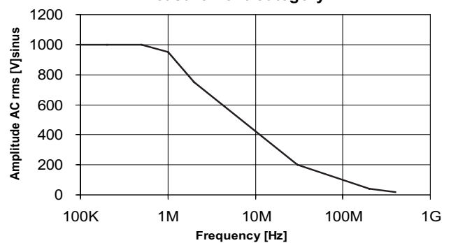
Typical Voltage Derating HVP120 Measurement Category I
